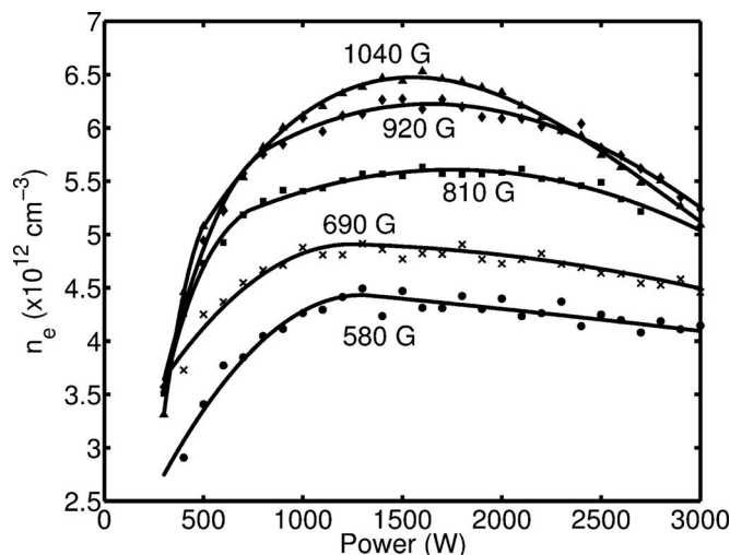
FIG. 10. Interferometer line-averaged n_e at z = 11 cm as a function of input rf power for source region magnetic fields of 580 G (circles), 690 G (crosses), 810 G (squares), 920 G (diamonds), and 1040 G (triangles). Nozzle configuration with 76 sccm flow rate.
